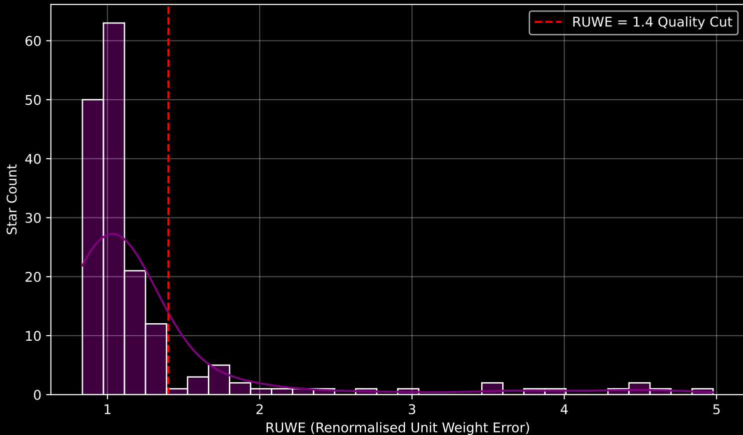
GAPOGEE DR17 Field [133+64_MGA] RUWE Distribution (n= 172)
