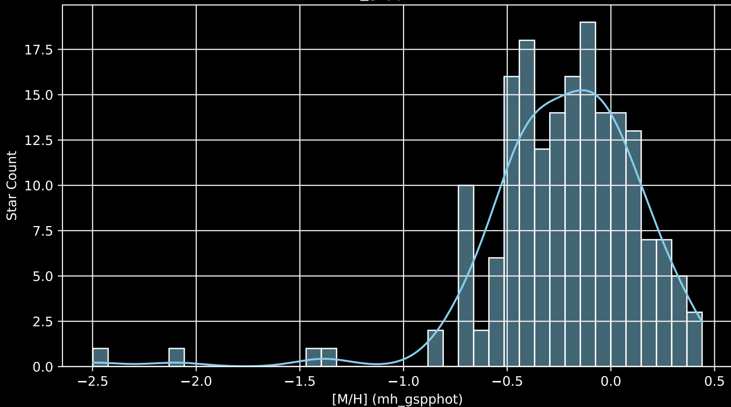
APOGEE DR17 Field: [133+64_MGA [M/H] (mh_gspphot) (n= 182)
