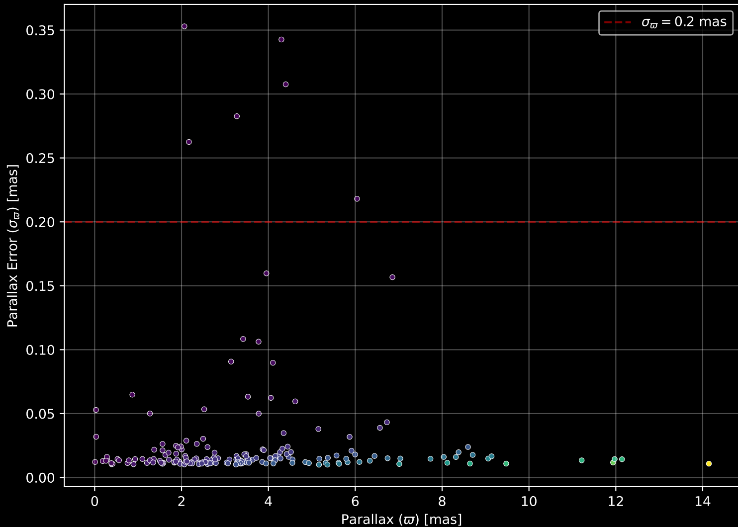
APOGEE DR17 Field: [133+64_MGA] Parallax Quality (n= 184)
