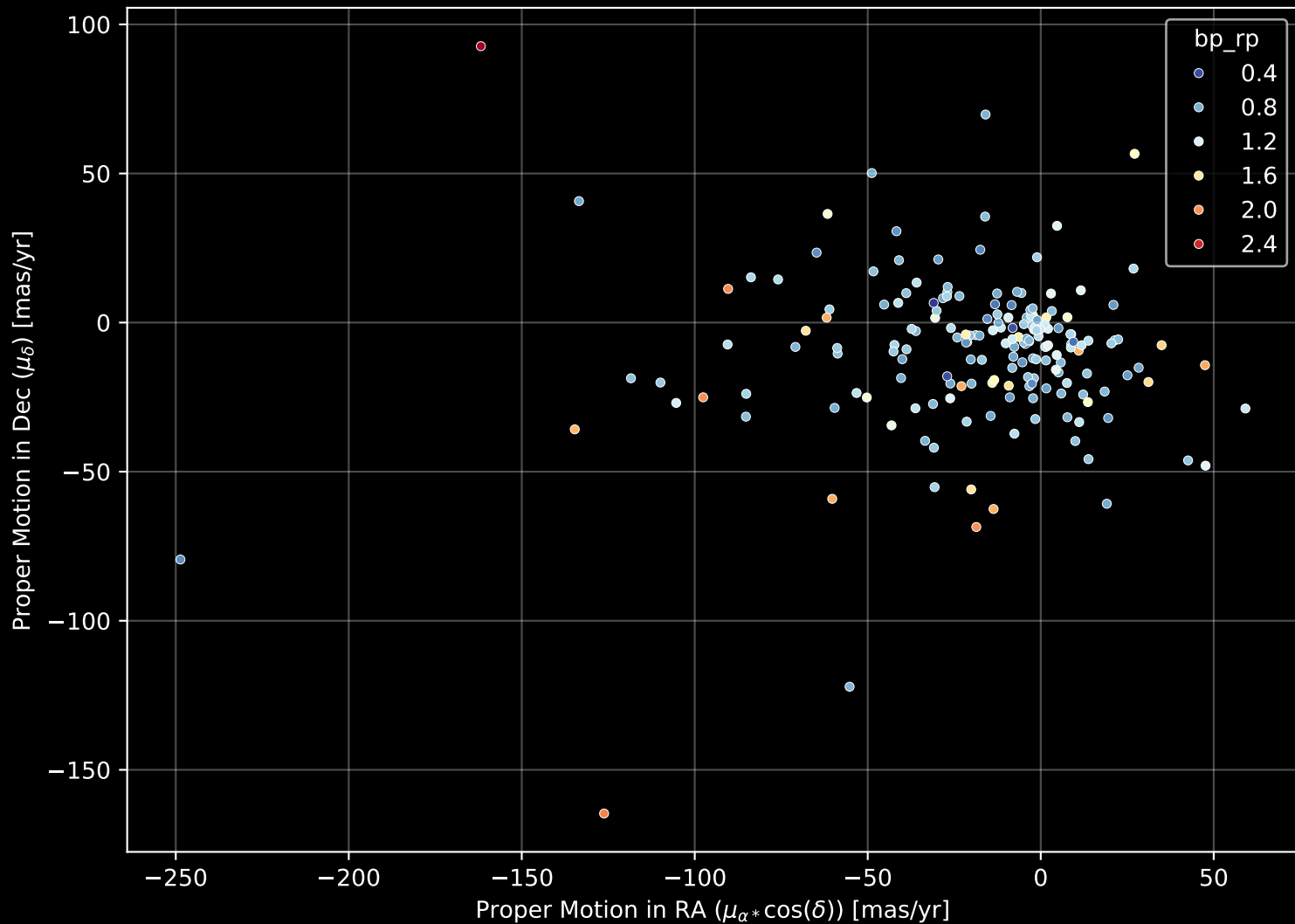
APOGEE DR17 Field: [133+64_MGA] Proper Motion Diagram (n= 184)
