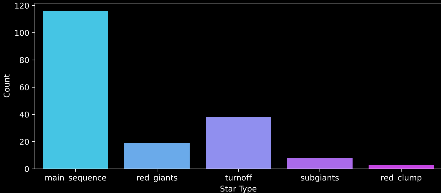
APOGEE DR17 Field: [133+64_MGA] Count plot of Star Type
