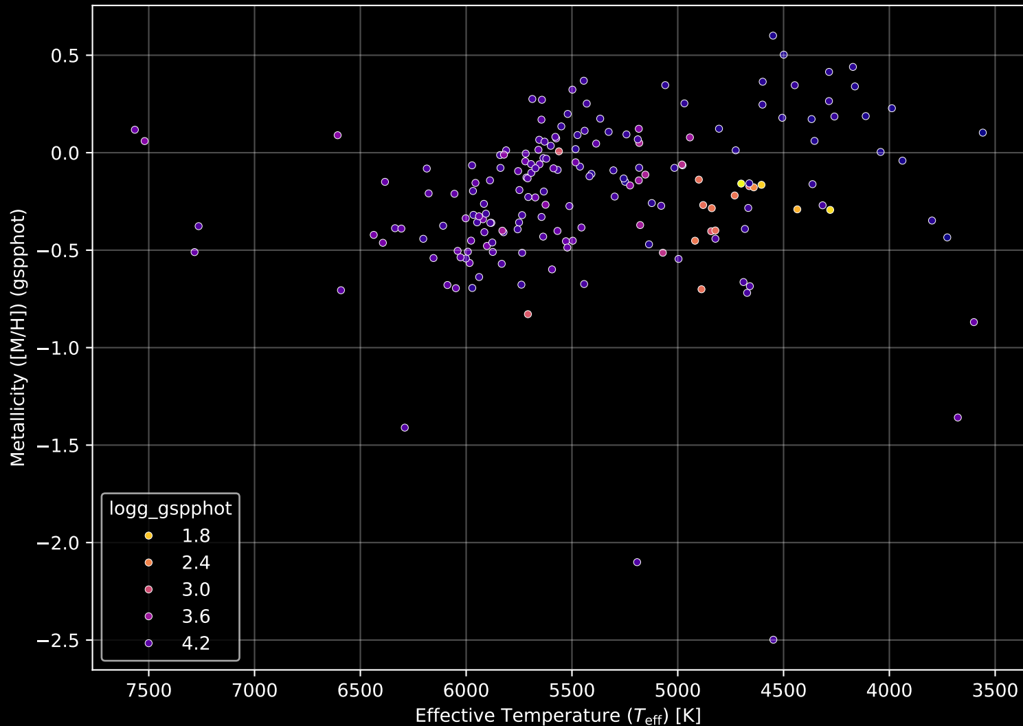
APOGEE DR17 Field: [133+64_MGA] Stellar Population Parameters (n= 184)
